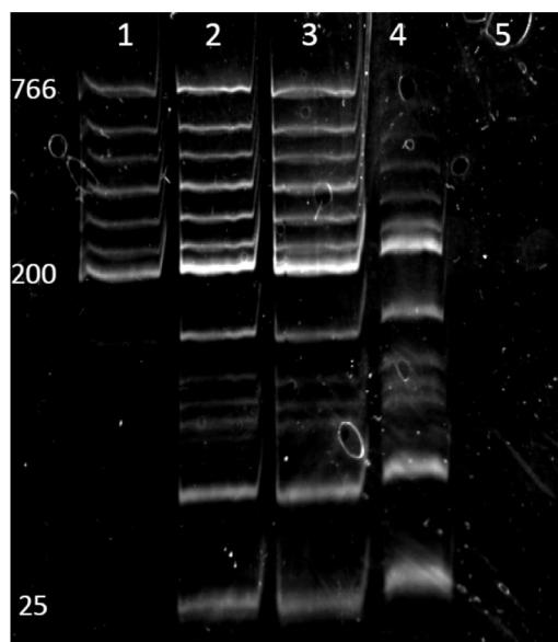
Fig. 6. A photograph of non-denaturing gel loaded with DNA samples from supernatant or re-suspended pellet after precipitation under various conditions. Lane 1: pellet from ethanol precipitation; lane 2: free DNA ladder; lane 3: pellet from SNP-assisted precipitation; lane 4: supernatant after ethanol precipitation; lane 5: supernatant after SNP-assisted precipitation.
