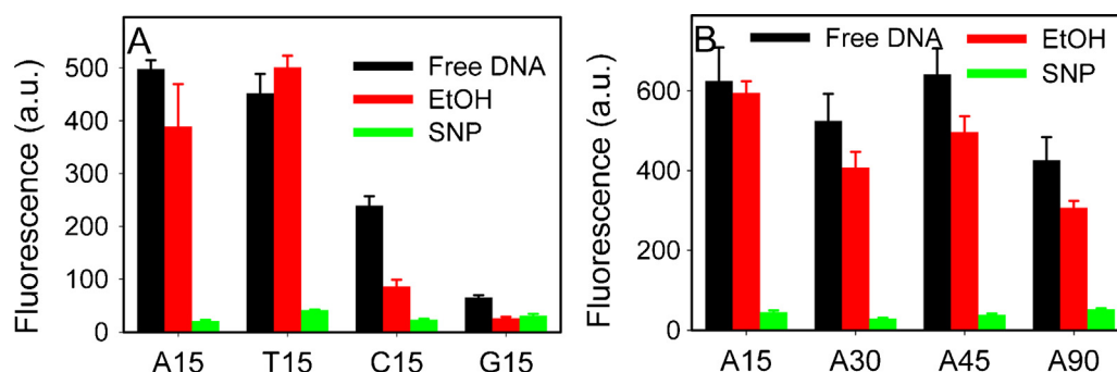
Fig. 4. Effect of DNA nucleotide composition (A) and length (B) on supernatant fluorescence after DNA precipitation.
