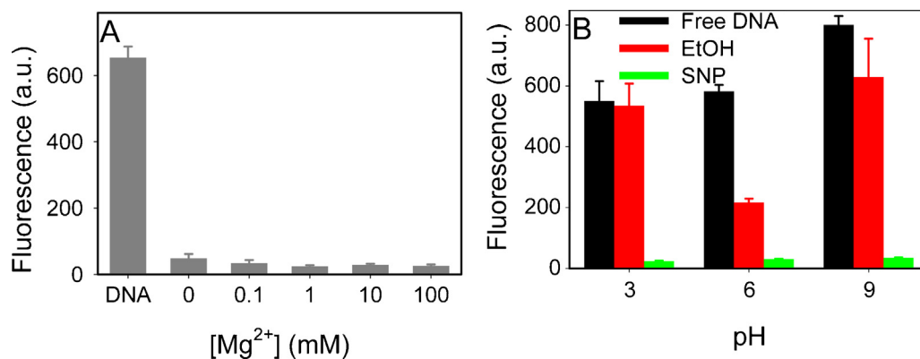
Fig. 5. Effect of salt concentration (A) and pH (B) on DNA precipitation by SNPs.
