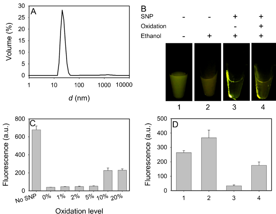
Fig. 2. (A) A DLS spectrum of a typical SNP sample used in this work (non-crosslinked). (B) Photographs of DNA precipitated under various conditions. Oxidation means carboxyl modified SNPs. (C) DNA precipitation measured as a function of SNP oxidation level. A lower supernatant fluorescence intensity means more precipitated DNA. (D) Supernatant fluorescence intensity of the samples in (B) indicating non-precipitated DNA concentration. The ethanol concentration was 67% in this experiment.
